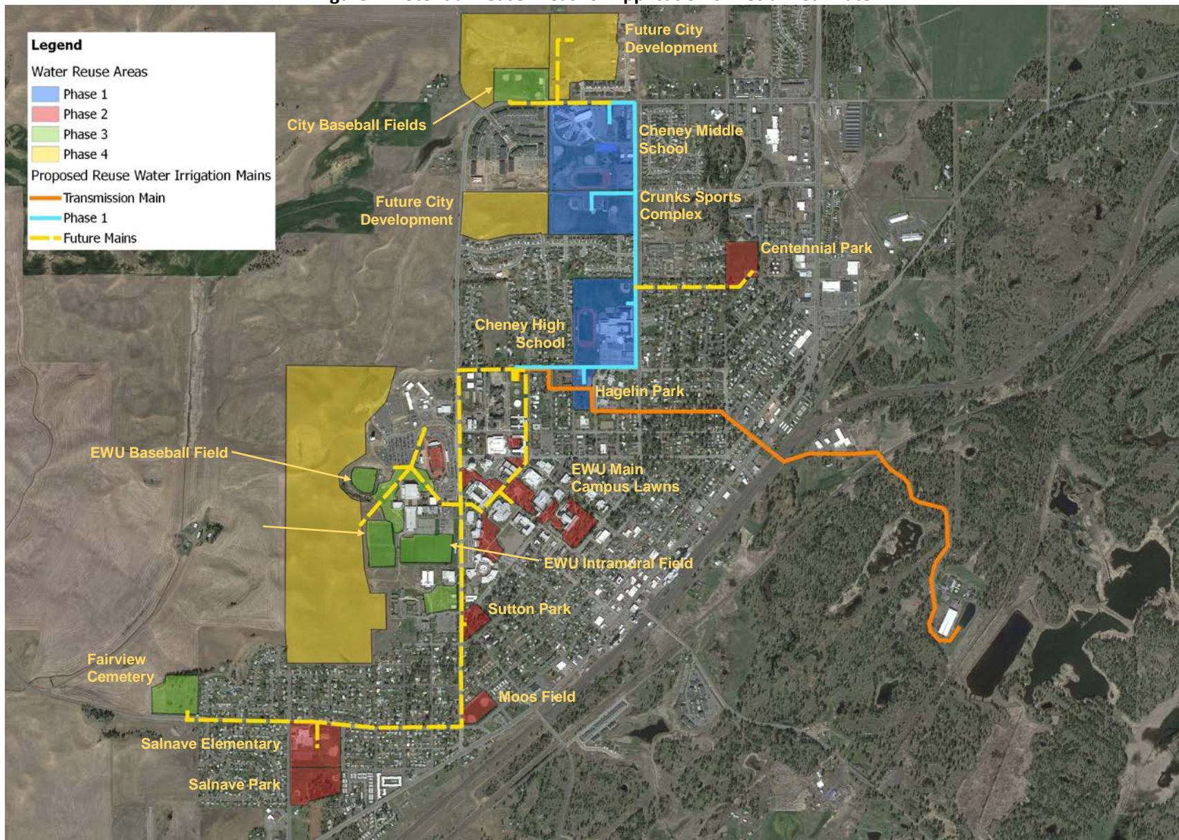
Figure 2. Potential Reuse Areas for Application of Reclaimed Water
